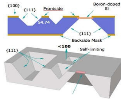
Figure 5: Illustration of shape of the etch profiles of a <100> oriented silicon substrate after immersion in an anisotropic wet etchant solution
