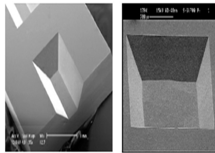
Figure 5: Illustration of shape of the etch profiles of a <100> oriented silicon substrate after immersion in an anisotropic wet etchant solution
