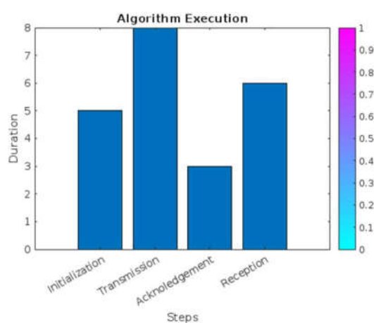
fig3: Algorithm Execution.
