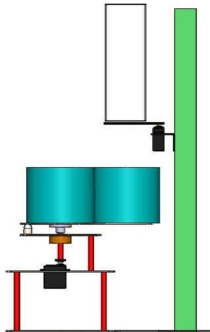
FIG 3.3: SIDE VIEW OF AUTOMATIC WASTE SEGREGATION SYSTEM
