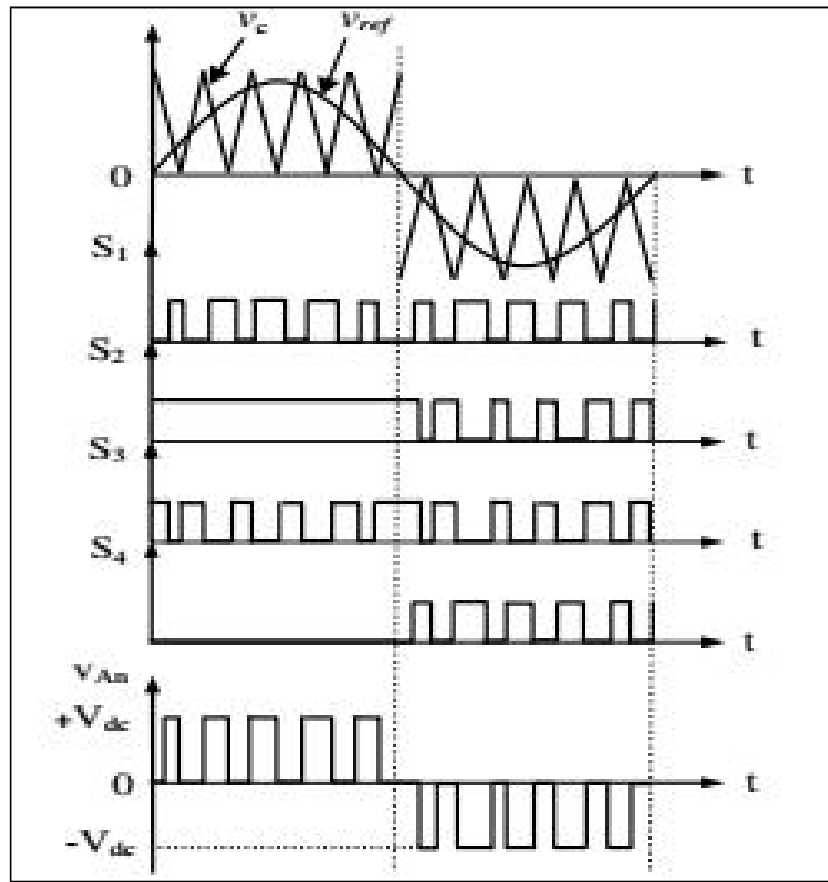
Figure 6: Unipolar SPWM method for proposed topology
